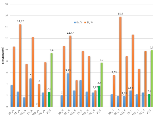
Fig. 15 Elongation of the foot ( \epsilon_s ) and the leg ( \epsilon_t ) of the viscose and tencel sock samples according to sock groups A, B and C
