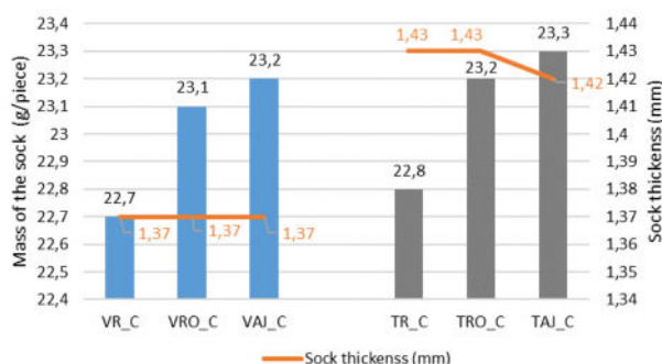
Fig. 12 Comparison between the sock mass and thickness of sample groups C
