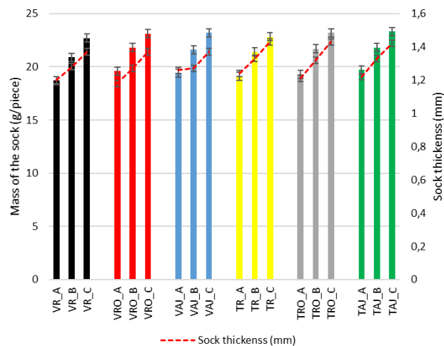
Fig. 9 Comparison of mass and thickness of socks
