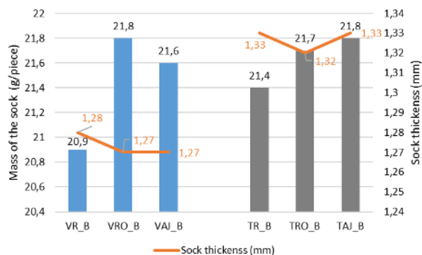
Fig. 11 Comparison between the sock mass and thickness of sample groups B
