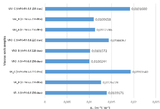
Fig. 17 Thermal resistance of viscose sock samples
