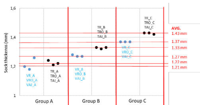
Fig. 13 Sock thickness per sample groups A, B and C
