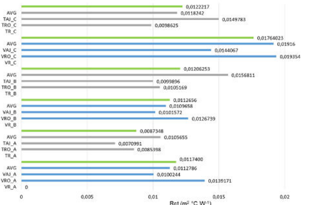
Fig. 20 Thermal resistance of viscose and Tencel socks of group A, B, C
