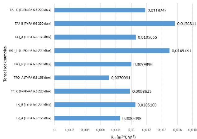
Fig. 18 Thermal resistance of tencel sock samples
