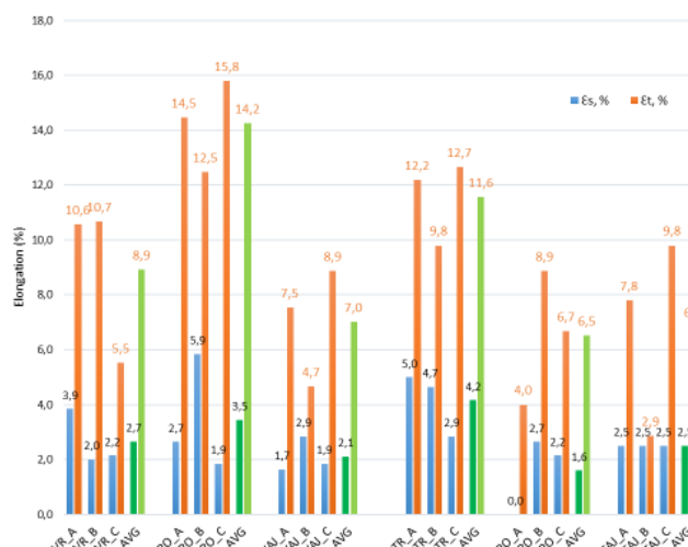
Fig. 16 Elongation of the foot ( \epsilon_s ) and leg ( \epsilon_t ) of viscose and tencel sock samples according to yarn type
