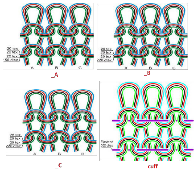
Fig. 1 View of the yarn in the structure of the leg and cuff of the sock; group of sock samples A, group of sock samples B, group of sock samples C
